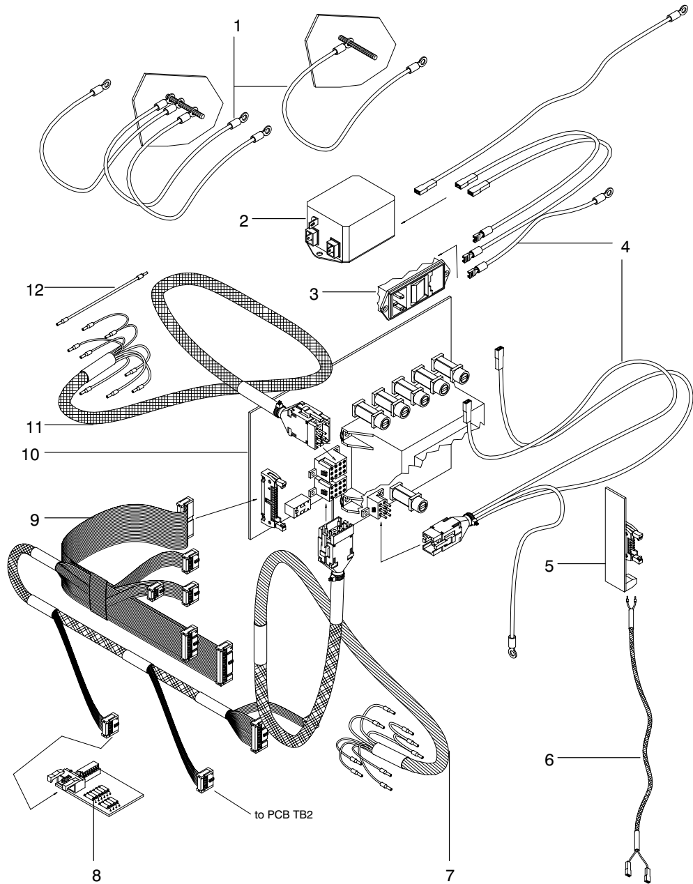
Figure 8-1. Oven Unit Group
